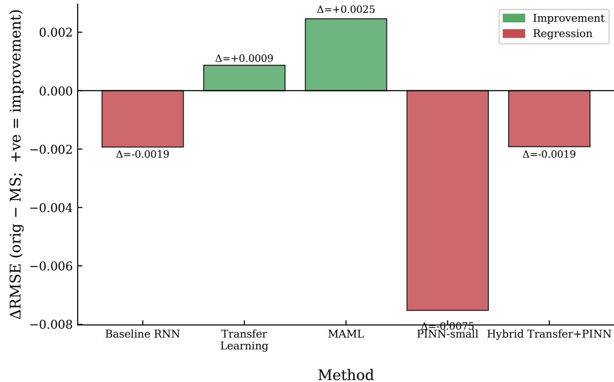
Duffing — Effect of Multi-Step Curriculum Training on RMSE
